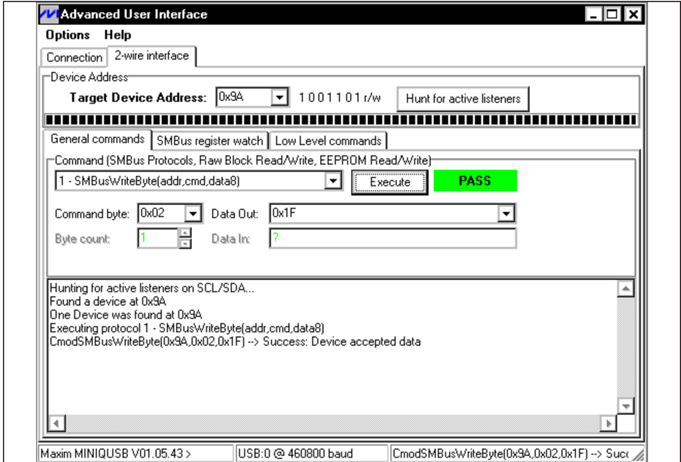
Figure 3. Simple Low-Level 2-Wire Interface
