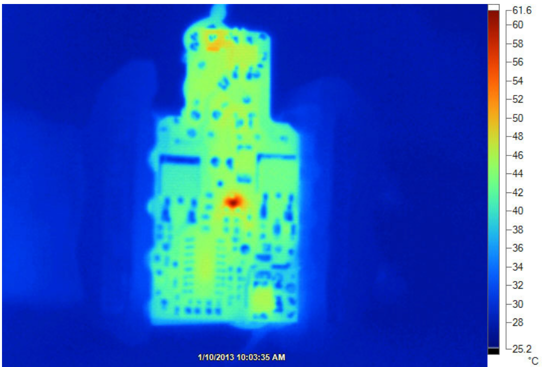
Figure 9. Bottom Thermal
